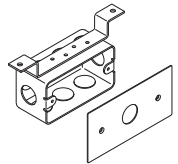
BFM-1-C Base Feed Kit
