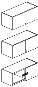
UEFS-LM UEKS-LM UEHS-LM Overhead Storage Unit, Standard Mount — Laminate Door
