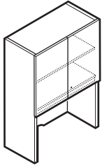
X4VL-NW X4VD-NW X5VL-NL X5VD-NL 30" and 36" widths
